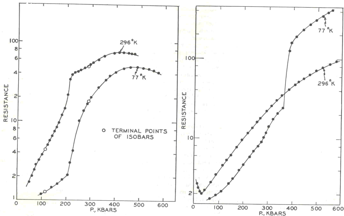
Fig. 9 (left). Resistance plotted against pressure for rubidium. Fig. 10 (right). Resistance plotted against pressure for potassium.
